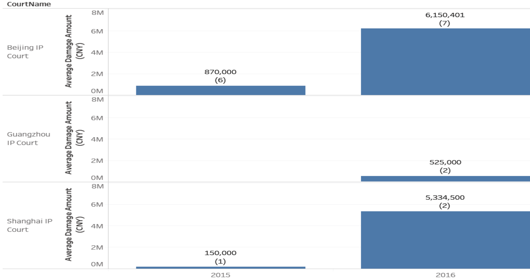
First Instance Average Damages By Year and IP Court
